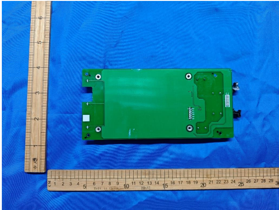
Fig. 17 -- PCB view 10
