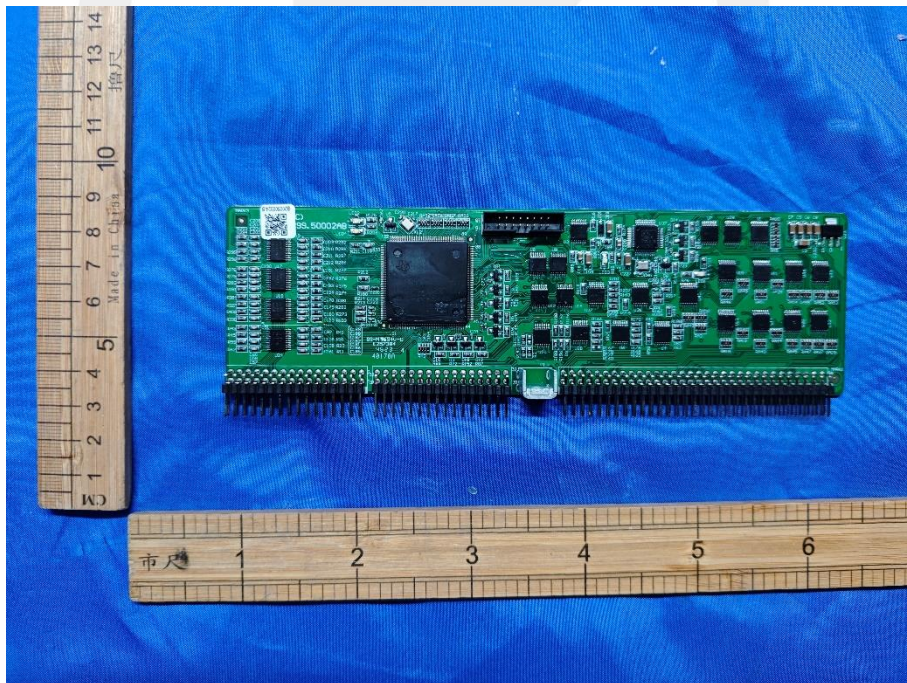
Fig. 20 -- PCB view 13
