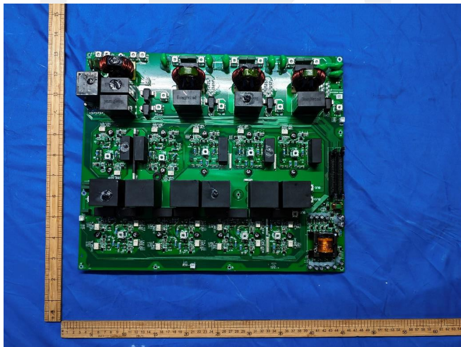
Fig. 10 -- PCB view 3
