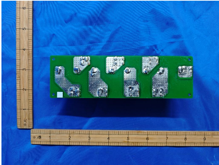
Fig. 19 -- PCB view 12
